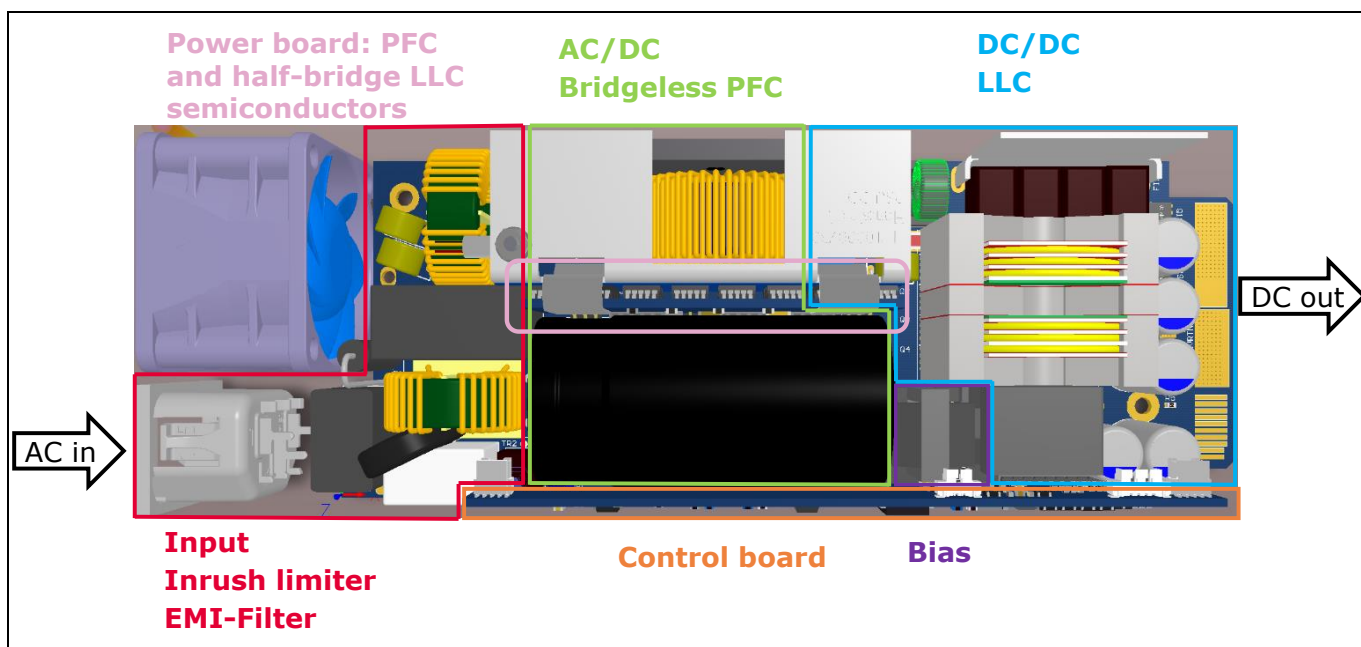
Figure 4 Placement of the different sections in the 1600 W PSU with Infineon DPAK CoolMOS™ and CoolSiC™
